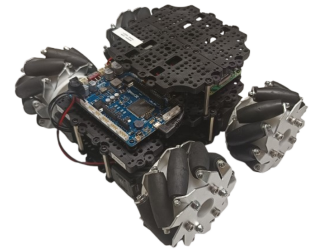
FIGURE 6.2 – TurtleBot Mecanum
