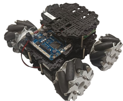
FIGURE 6.1 – TurtleBot Mecanum
