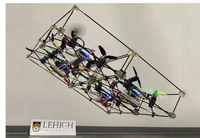
FIGURE 2.1 – Système ModQuad [2].
