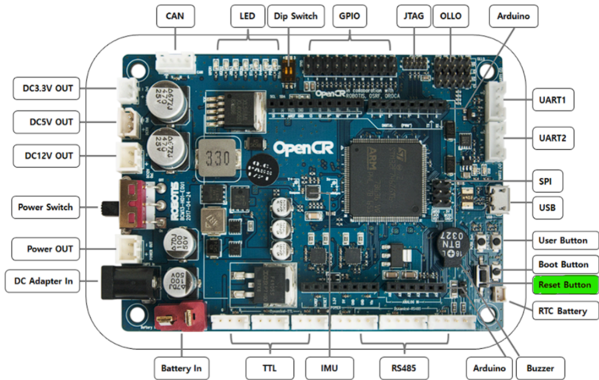
FIGURE 3.3 – Pinout OpenCR
