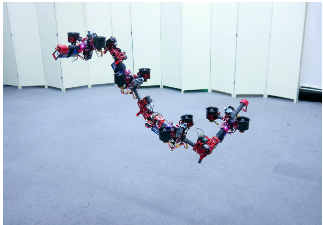
FIGURE 4.2 – Drone DRAGON [1]
