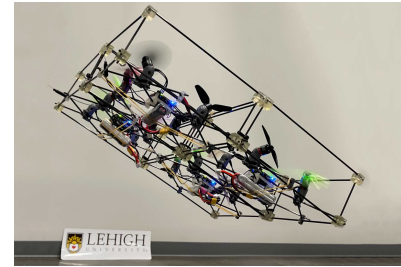
FIGURE 2.1 – Système ModQuad [2].
