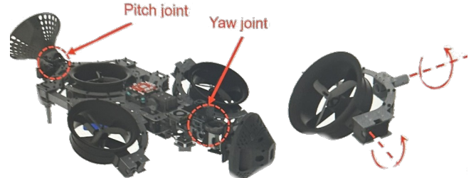
FIGURE 4.7 – Système LEGION [6]
