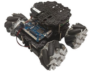
FIGURE 6.2 – TurtleBot Mecanum
