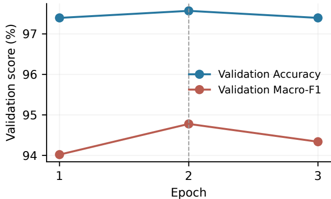
(b) Best checkpoint: epoch 2
