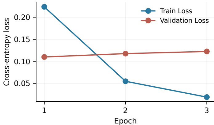
(a) Optimization and generalization
