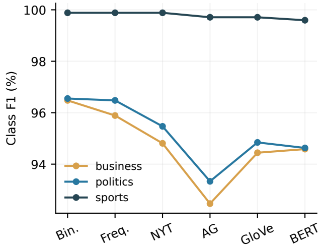
(b) Minority-class performance
