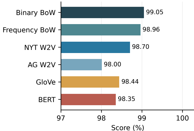
(a) Accuracy
