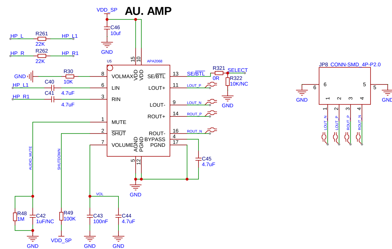
Dual channel power amplifier
