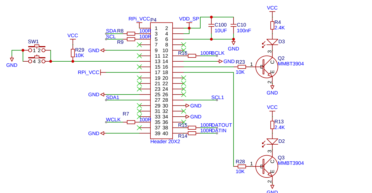
RPi-20*2 PinOut
