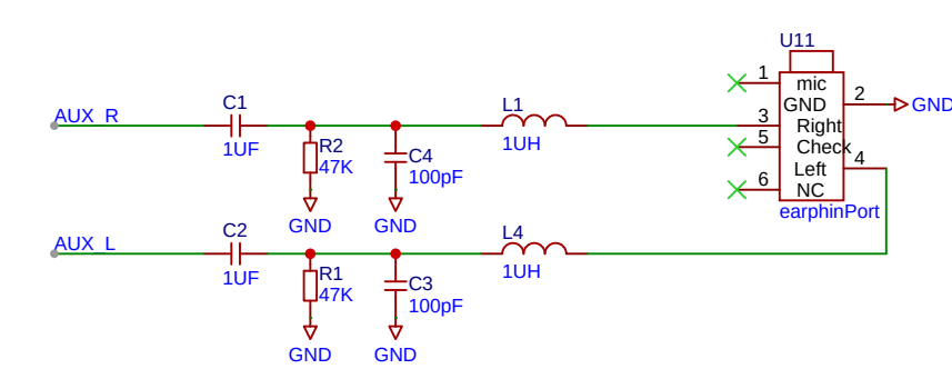
3.5mm AUX
