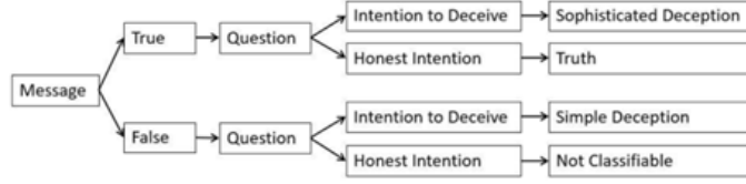
Figure 3: Sender-Receiver Game
