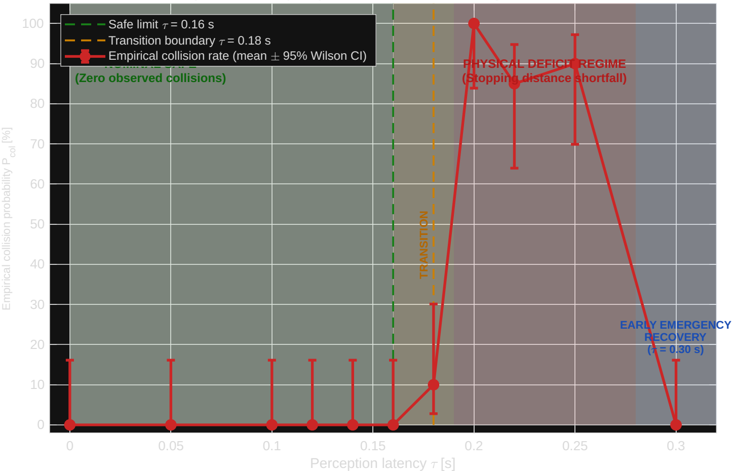
Empirical latency-dependent collision envelope of CA-CRC
