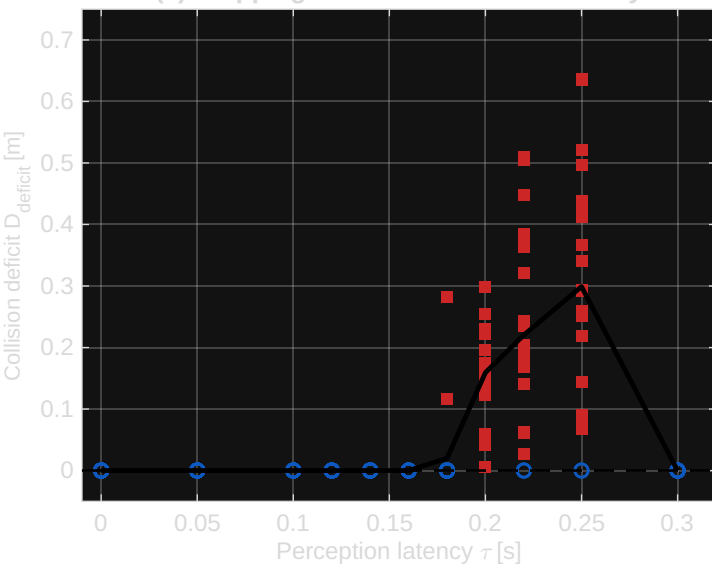
(c) Stopping distance deficit vs. latency
