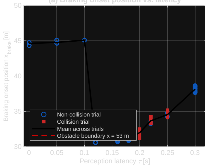
(a) Braking onset position vs. latency
