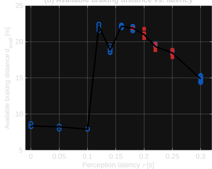
(b) Available braking distance vs. latency
