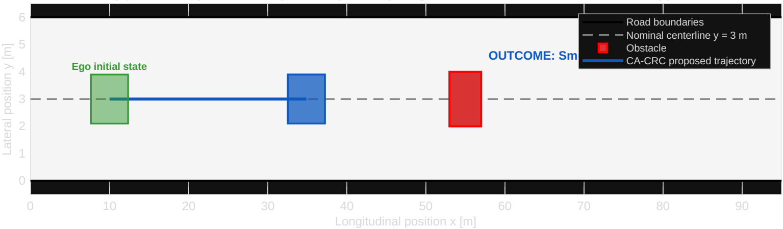
(b) CA-CRC (PROPOSED): Free-space topological evaluation → Smooth lateral bypass
