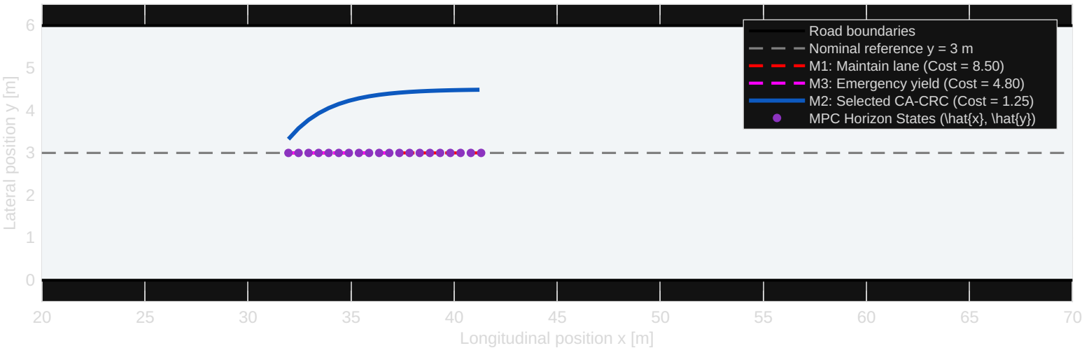
(a) Candidate Ego Maneuvers & Selected MPC Optimization Horizon
