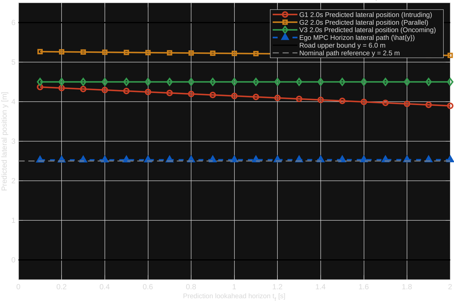
Dynamic Agent Spatio-Temporal Prediction Horizons & Ego Reachable Space (Lookahead N_p = 20, 2.0s )
