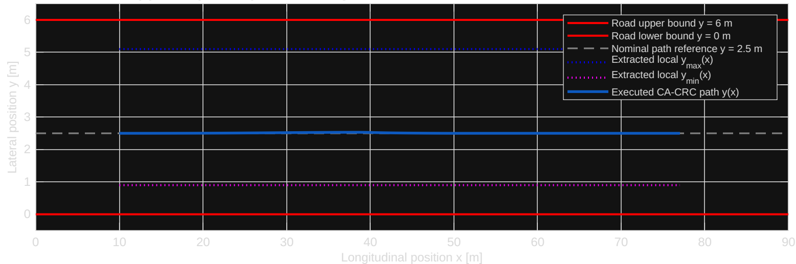
(a) FreeSpaceMap Extracted Dynamic Drivable Corridor Bounds & Executed Path
