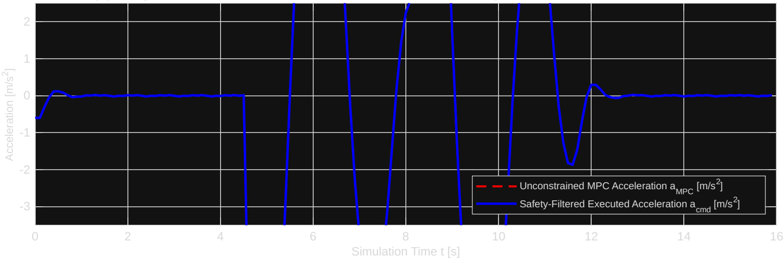
(b) Longitudinal Control Audit: Unconstrained MPC vs Safety-Filtered Acceleration Command
