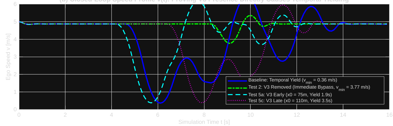
(b) Closed-Loop Speed Profile v(t) : Proving V3 Presence Directly Causes Temporal Yielding
