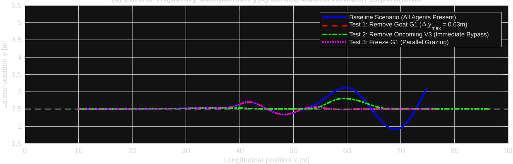
(a) Lateral Trajectory Comparison y(x) across Causal Ablation Experiments
