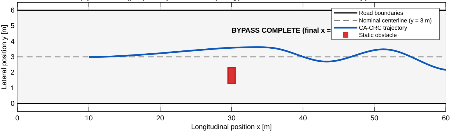
(b) CA-CRC (proposed): corridor topology evaluation \rightarrow smooth lateral bypass
