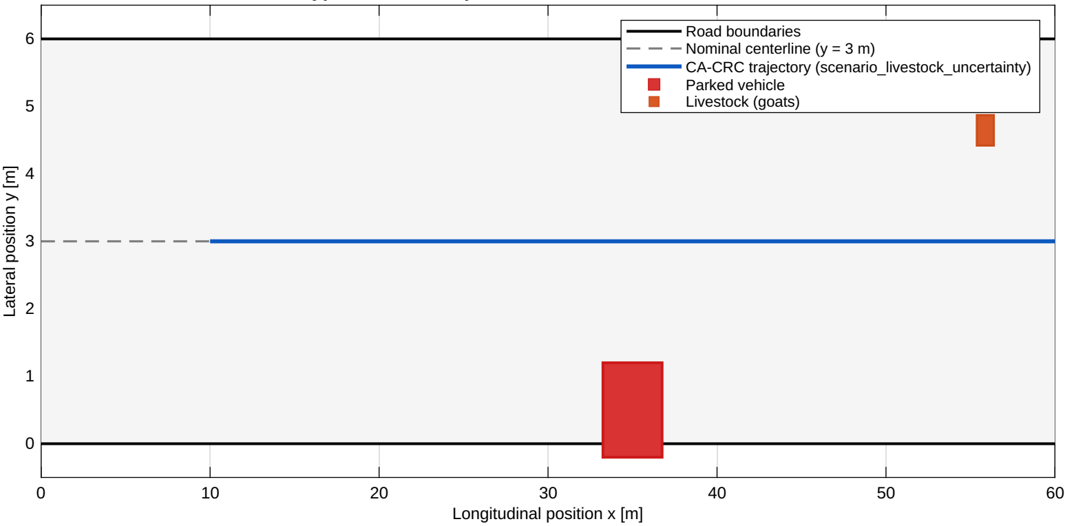
CA-CRC bypass: roadside parked-vehicle + livestock-intrusion scenario
