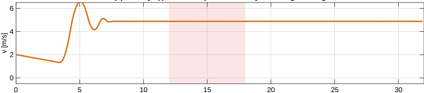
(b) Velocity v(t) -- smooth speed control & yield during crossing
