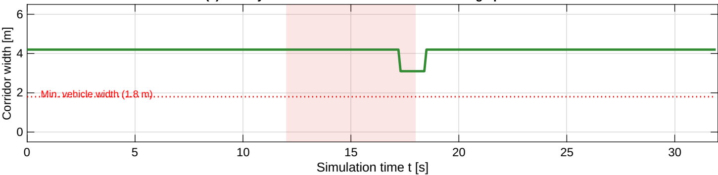
(c) Locally extracted drivable corridor width at ego position
