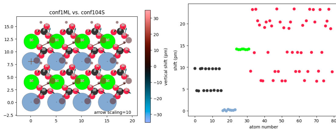
FIG. S5. (a) Top layer of the DFT-calculated dolomite (104)^S and \text{H}_2\text{O}/\text{dolomite}(104)^S surface. Numbers denote the absolute shift between the (104)^S and the respective \text{H}_2\text{O}/\text{dolomite}(104)^S surface models. (b) Absolute shifts for all atoms in the top layer. Colours are element-specific and identical to those in (a).
