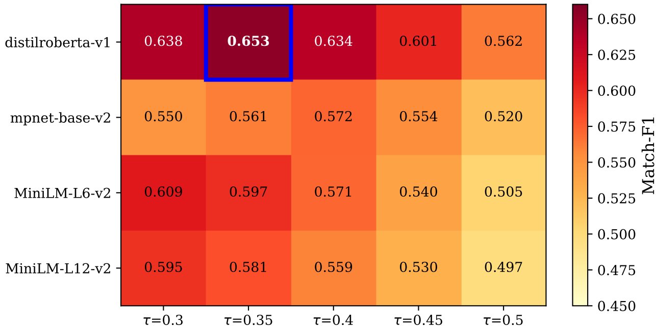
Match-F1 Ablation: Encoder \times Threshold
