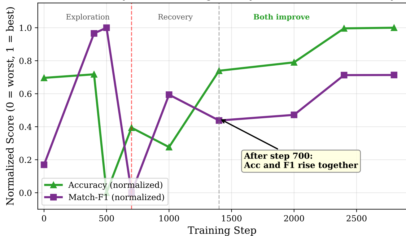
CPR: Accuracy and Reasoning Quality Co-evolve After Recovery
