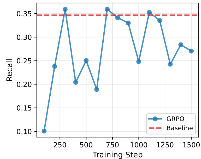
(e) Recall
