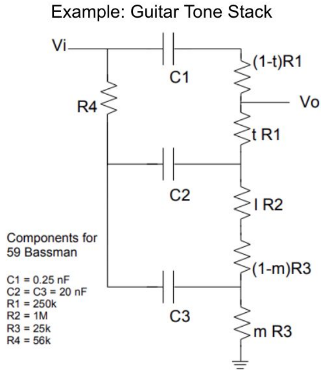
Figure 1: Tone stack circuit with component values.
