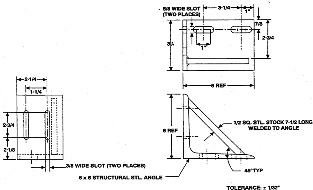
FIGURE No. 6 SUPPORT BRACKET LUMBER TEST FIXTURE
