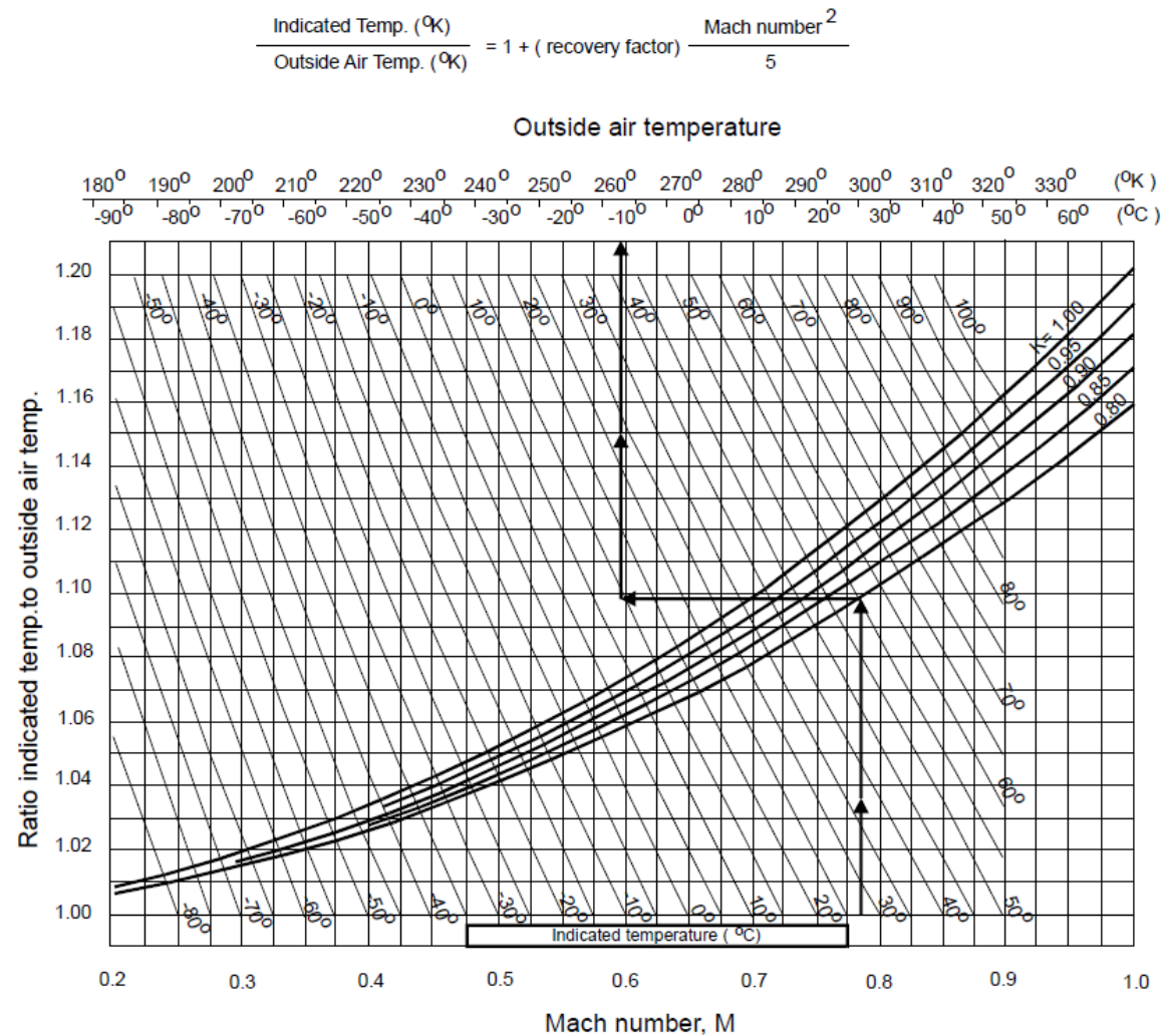
Figure 7 – TEMPERATURE RAM RISE
