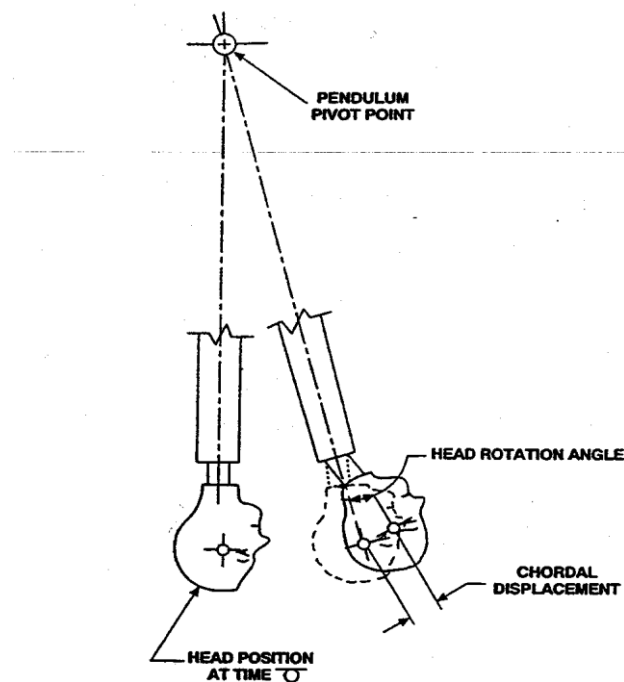
FIGURE No. 3 NECK COMPONENT TEST
