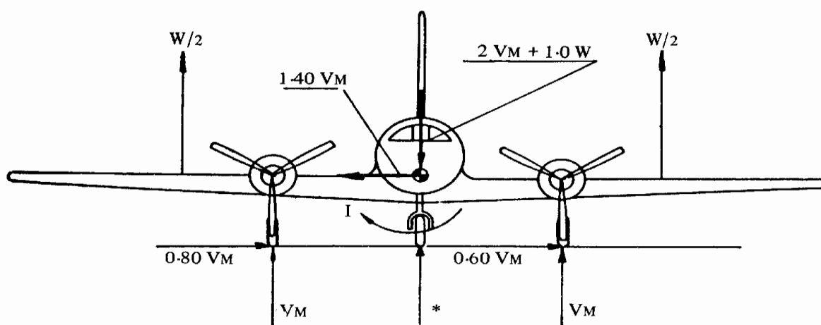
FIGURE 4 ONE-WHEEL LANDING
