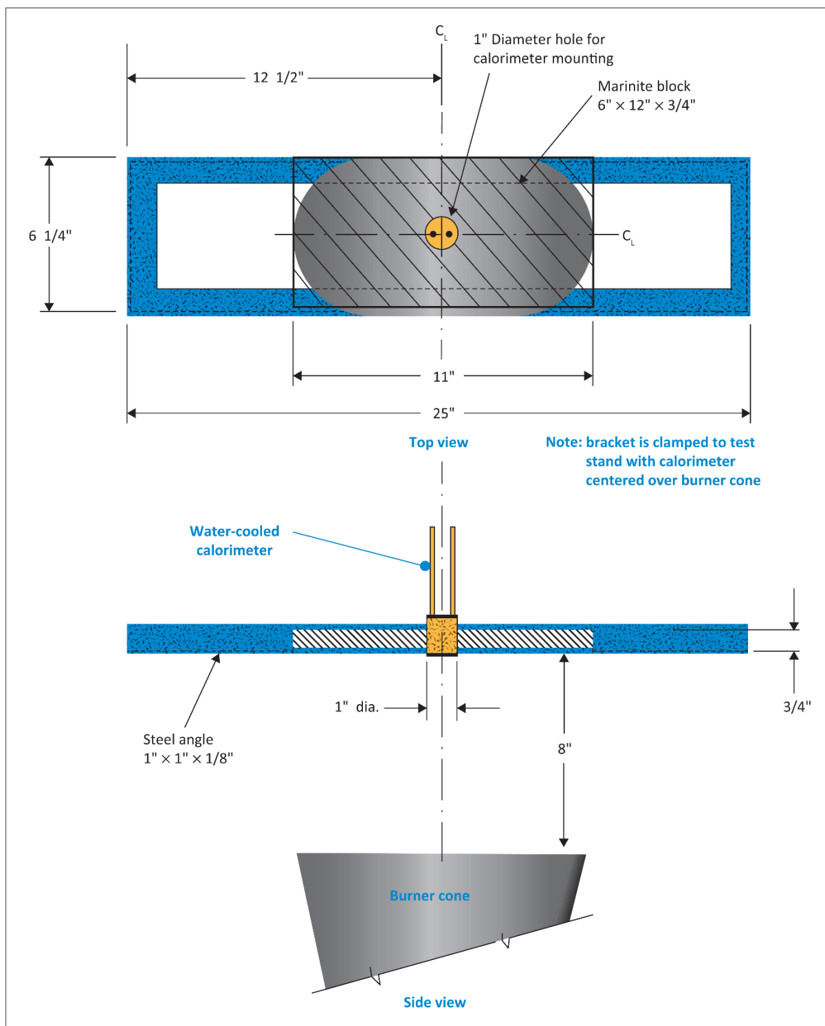
FIGURE 2 CALORIMETER BRACKET
