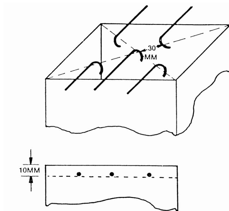
FIGURE 5. THERMOCOUPLE POSITION
