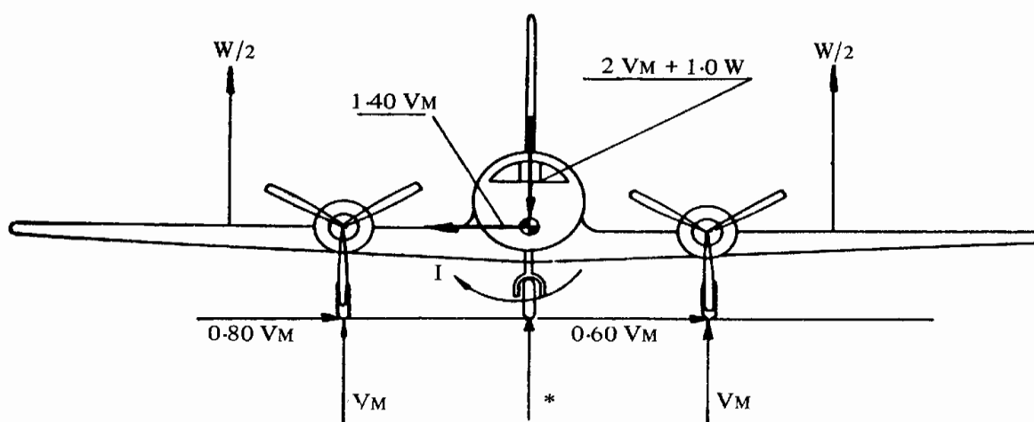
FIGURE 4 ONE-WHEEL LANDING
