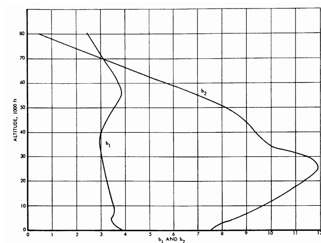
FIGURE 2 – b_1 AND b_2 VALUES AMC 25.345(a)
