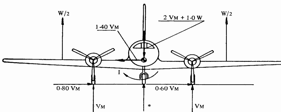
FIGURE 4 ONE-WHEEL LANDING
