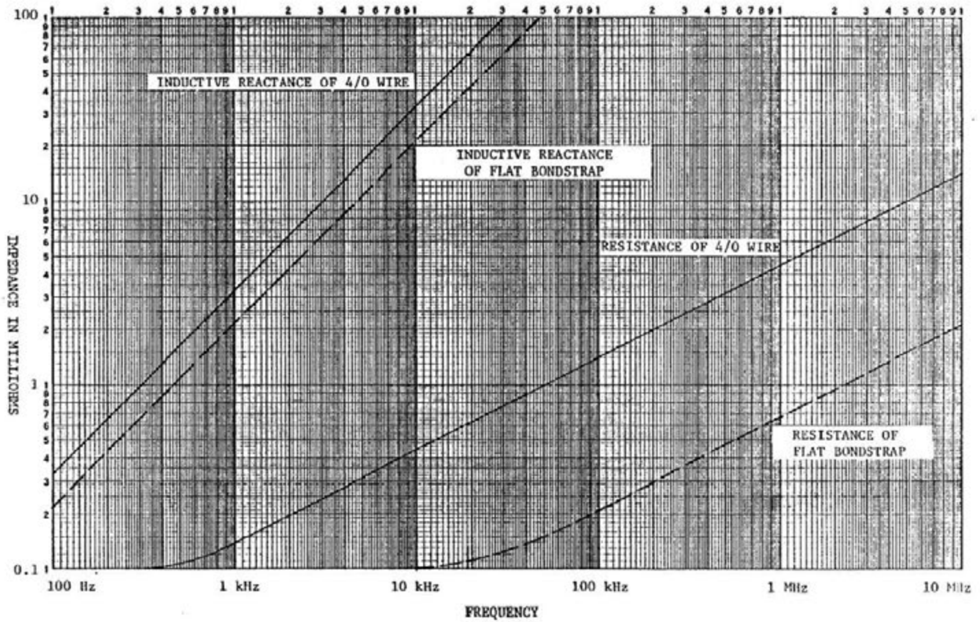
FIGURE 32 - Plot Comparing Relative Magnitudes of Resistive and Inductive Components of Wire Impedance
