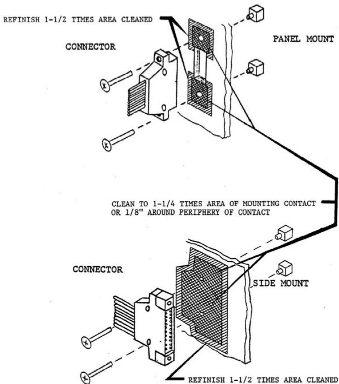
FIGURE 17 - Methods of Bonding Metal Connectors to Attaching Part
