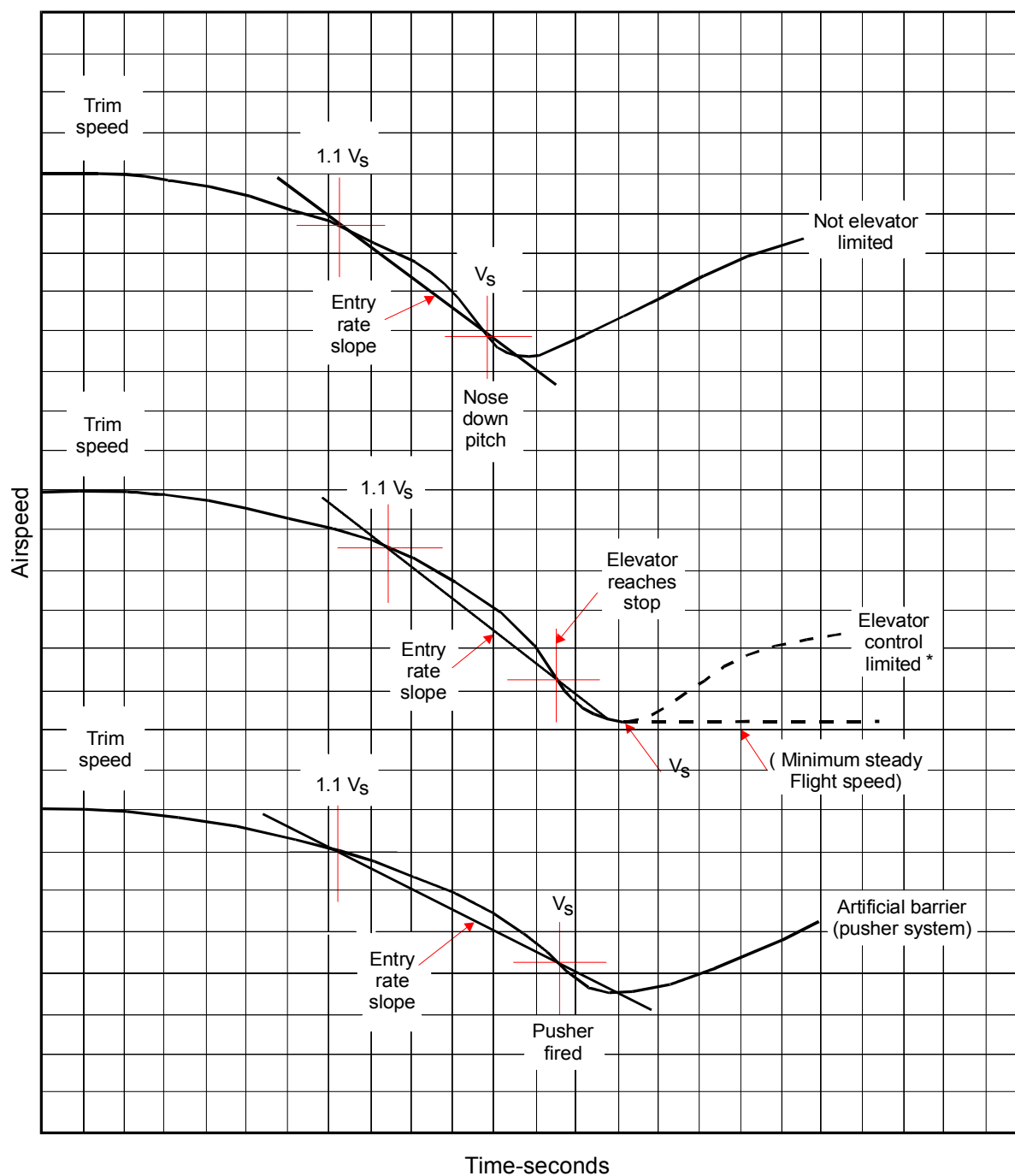
Figure 17-1 STALL SPEED
