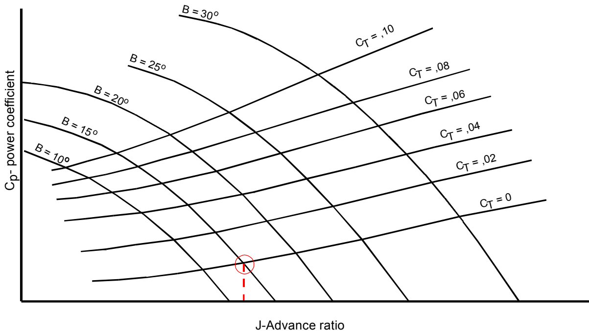
Figure 17-2 PROPELLER COEFFICIENTS
