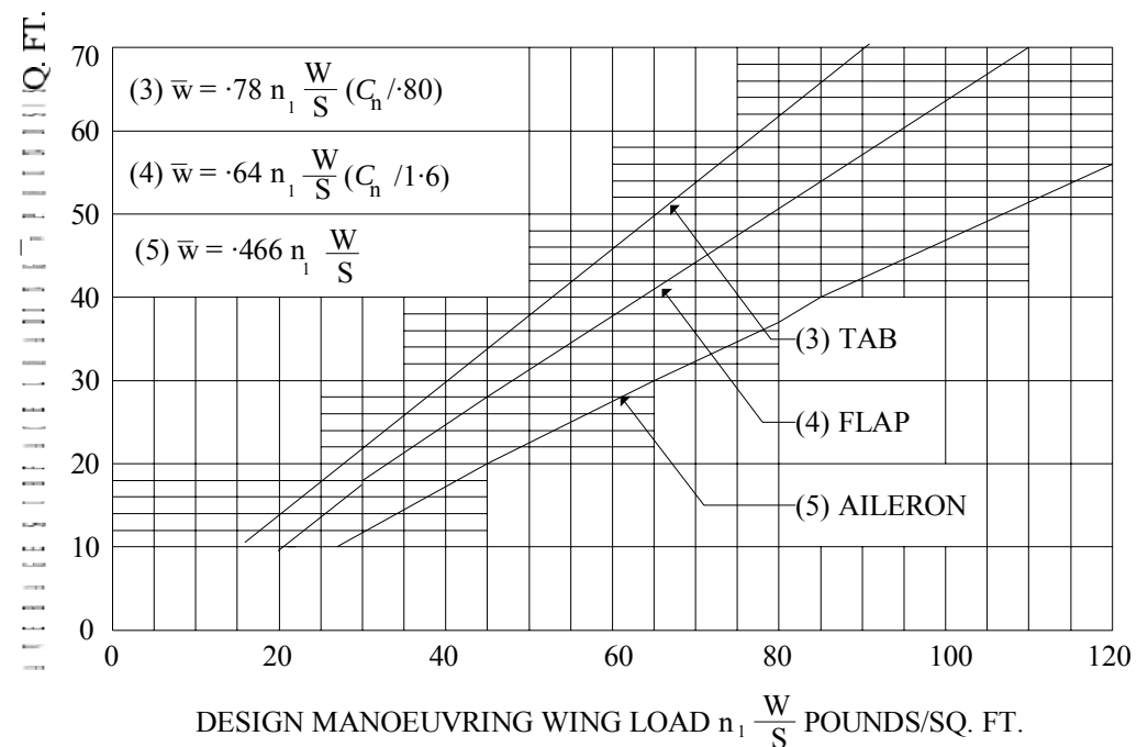
FIGURE A6 - Average limit control surface loading.
