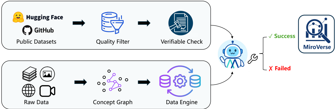
Figure 3: Overview of the data construction pipeline. Public datasets from platforms such as HuggingFace and GitHub are filtered and verified, while raw internet data are processed through knowledge graph generation and a data engine. The resulting QA pairs from both sources are then converted into agentic trajectories, forming the complete MiroVerse v1.0 dataset used for training MiroThinker v1.0.
