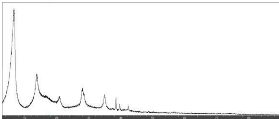
Mo 2 TiC 2 T x single-/few-layer powder — XRD. Representative characterization; not lot-specific. Non-data annotation removed; diffraction trace and axes otherwise unchanged.
