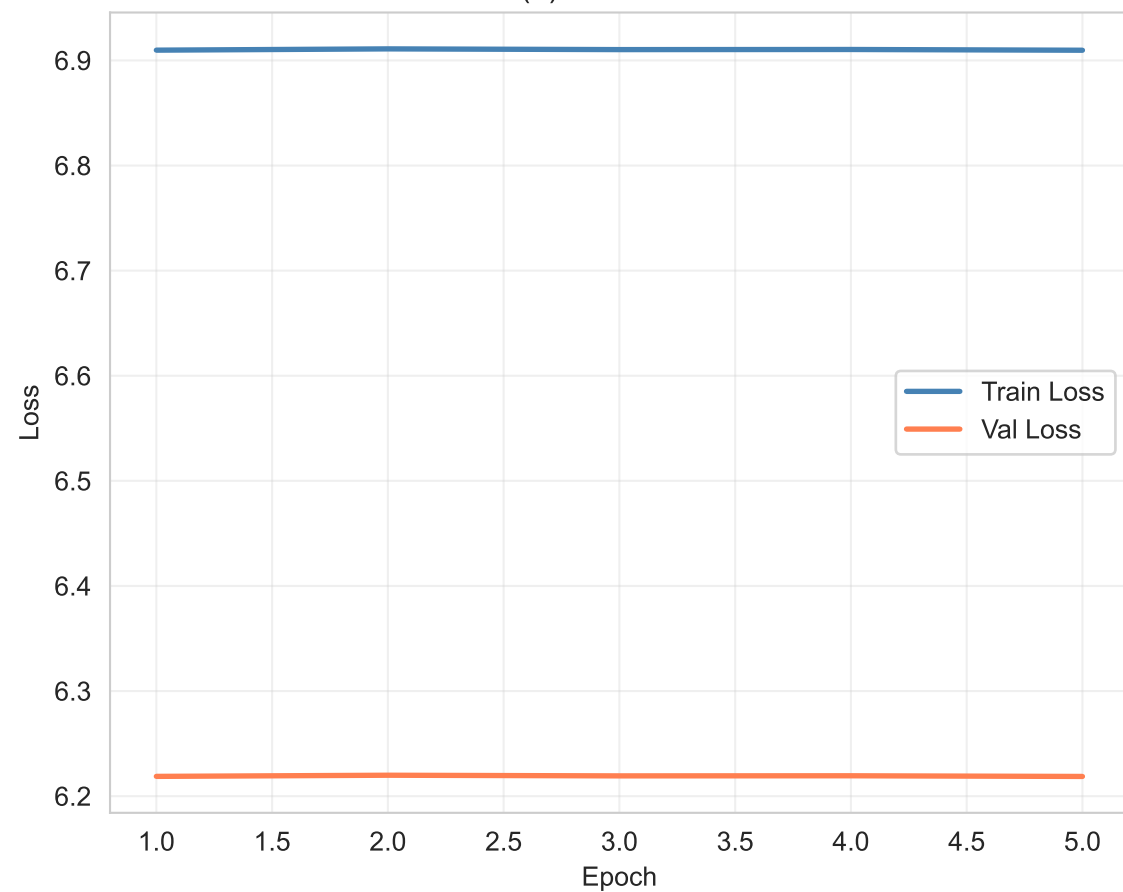
(c) RNN-T
