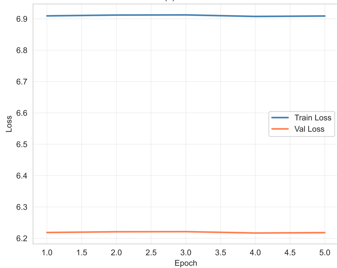
(c) RNN-T
