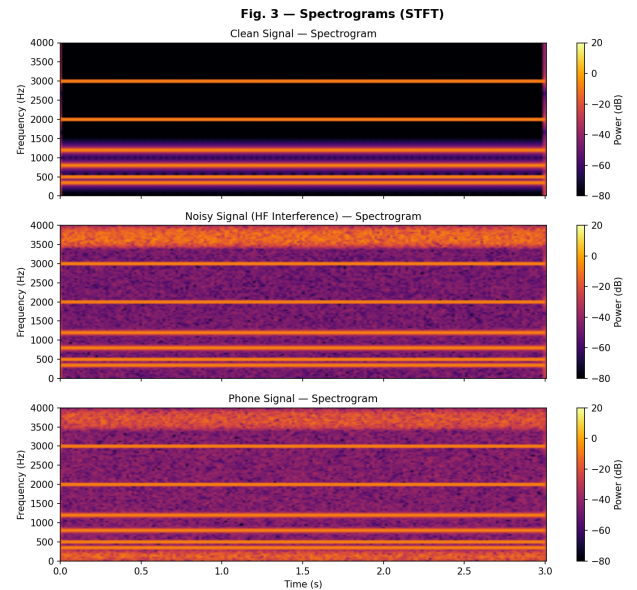
Fig. 3. Spectrograms (STFT) of the three signals. Horizontal bands are the tonal components.
