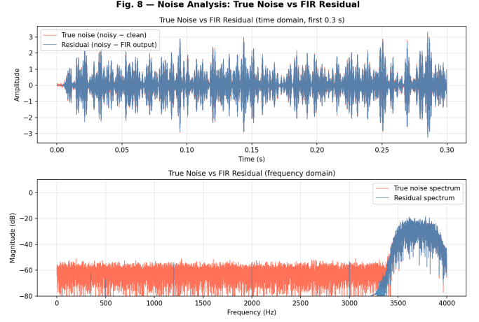
Fig. 8. True AWGN noise vs FIR filter residual in time and frequency domains.
