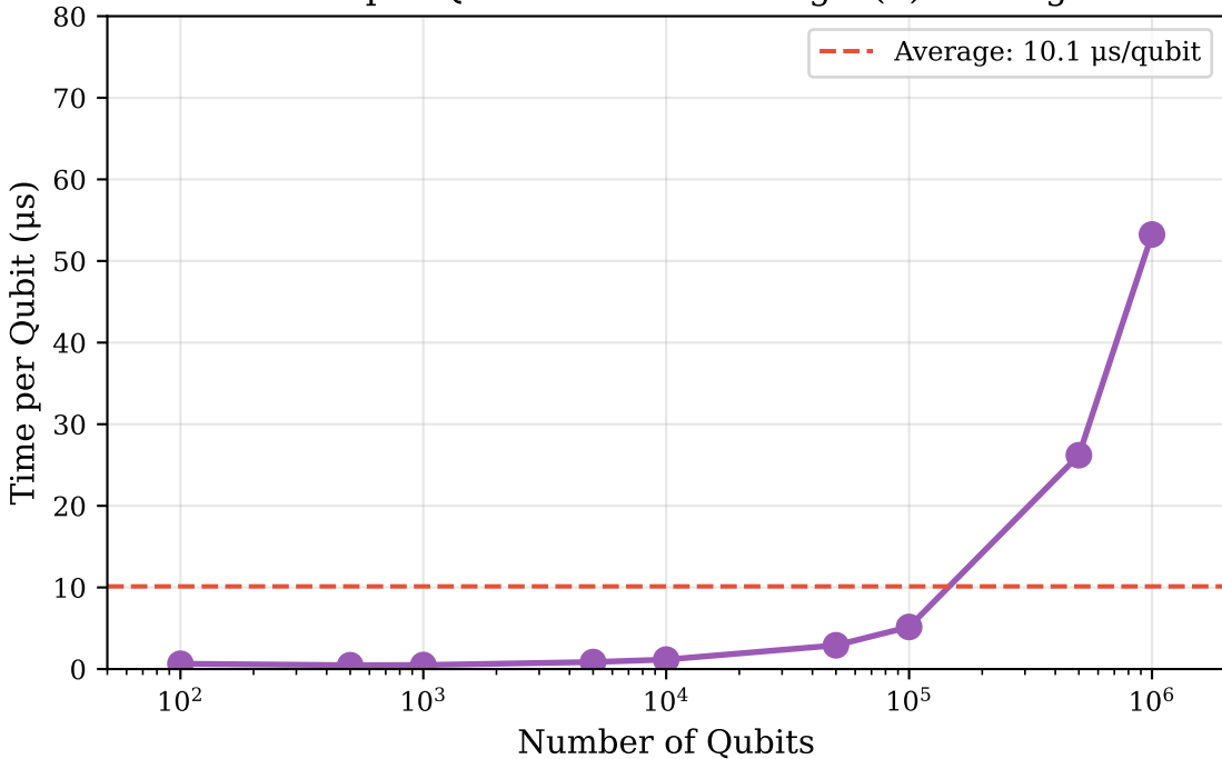
Time per Qubit: Demonstrating O(n) Scaling
