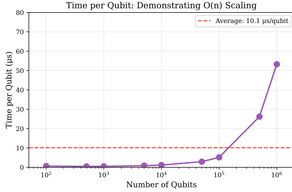
Figure 6: Time per qubit vs. qubit count. For small n , fixed overhead dominates; as n grows, BigInt arithmetic overhead causes per-qubit cost to increase from \sim 1 \mu\text{s} to \sim 53 \mu\text{s} at 10^6 qubits. This reflects O(n^{1.5}) empirical scaling rather than theoretical O(n) .
