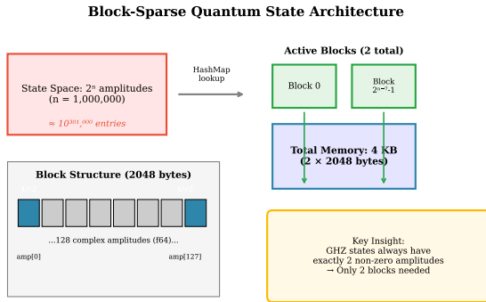
Figure 1: Block-sparse architecture. A HashMap maps block IDs to fixed-size blocks of 128 complex amplitudes. For GHZ states, only two blocks are allocated regardless of qubit count n , achieving O(1) memory for this state class.
