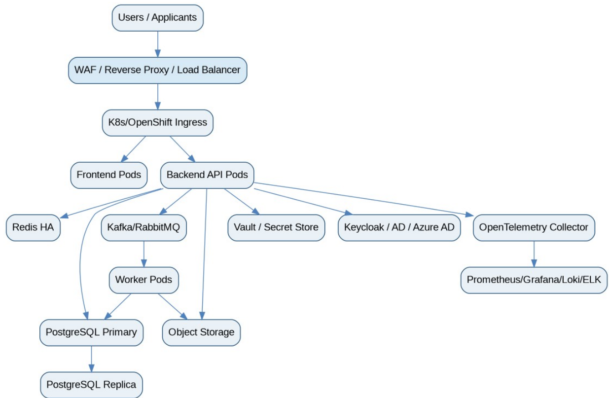
Figure 9 - Recommended production deployment topology.
