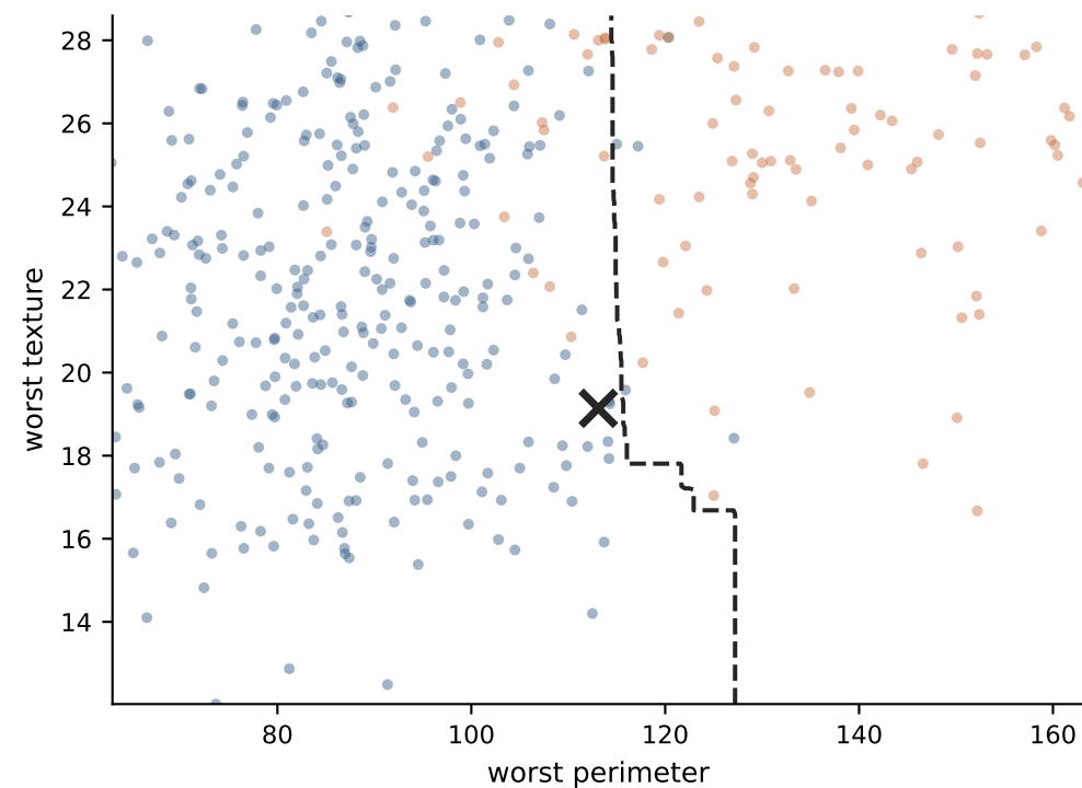
A · the black-box model
