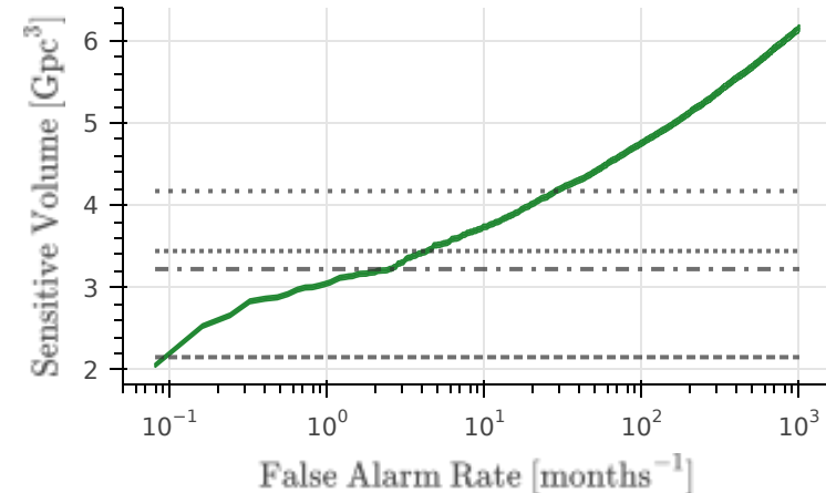
Log Normal m_1 = 20, m_2 = 20
