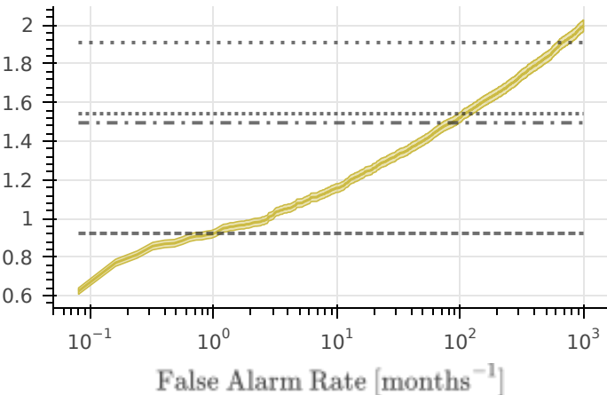
Log Normal m_1 = 20, m_2 = 10
