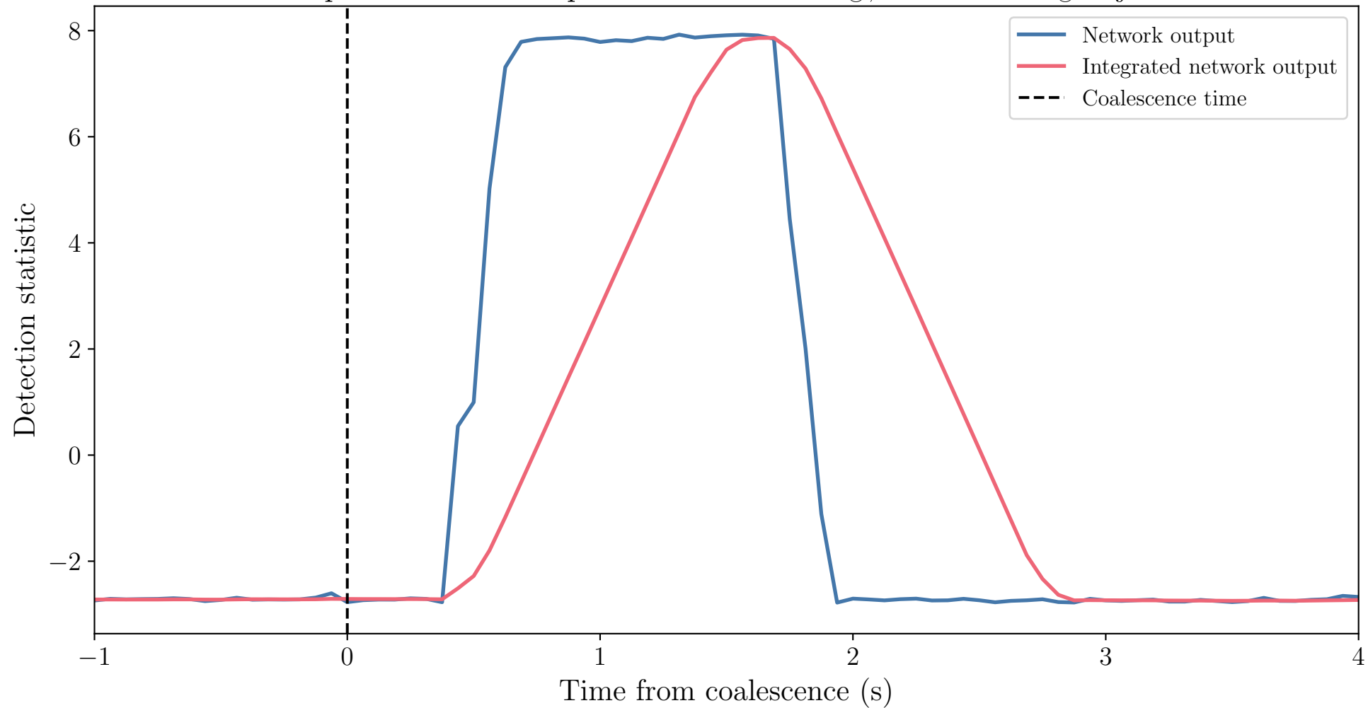
Example Network Output for m_1 = 35 M_\odot , m_2 = 35 M_\odot Injection
