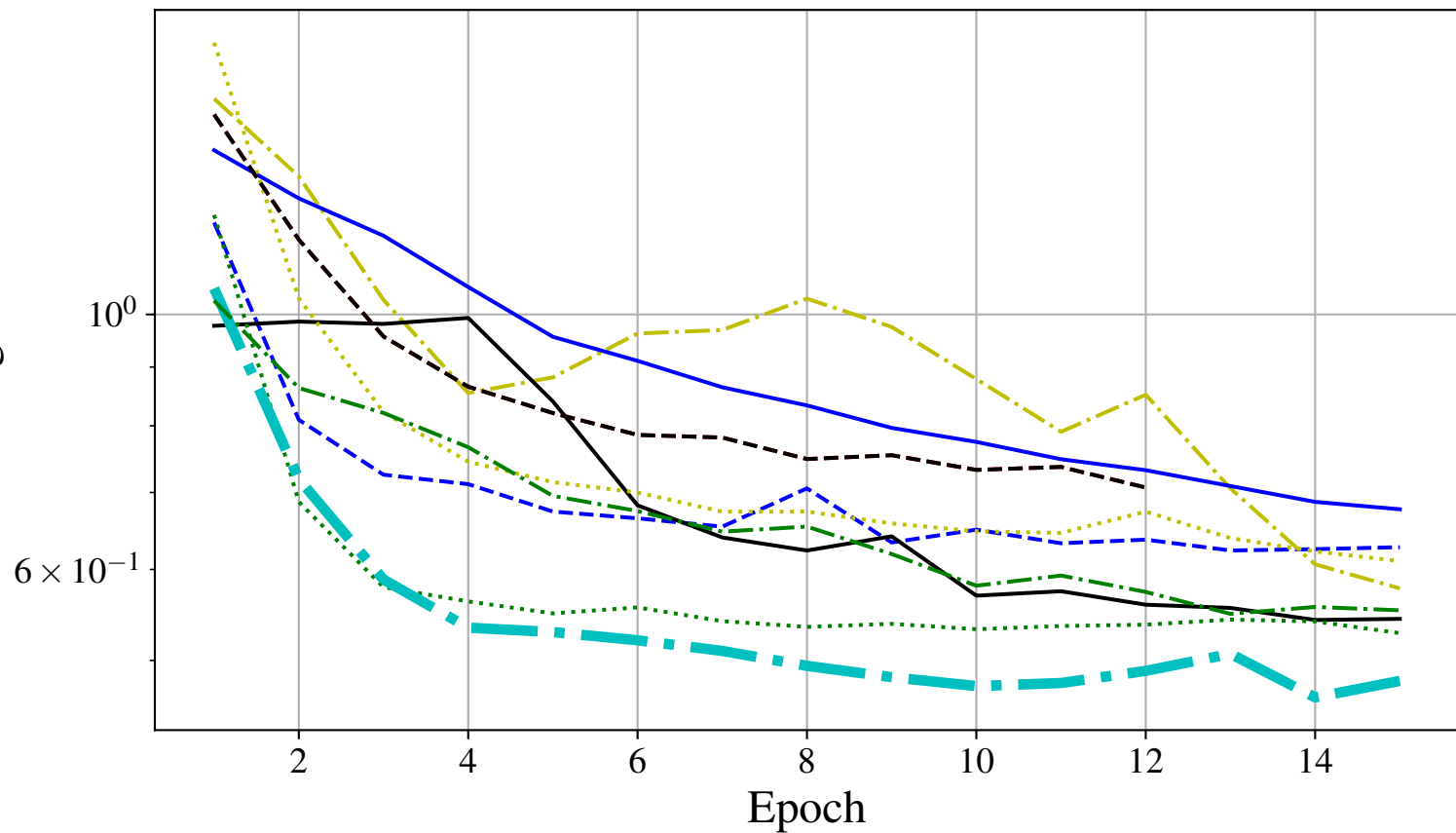
VICReg Loss
