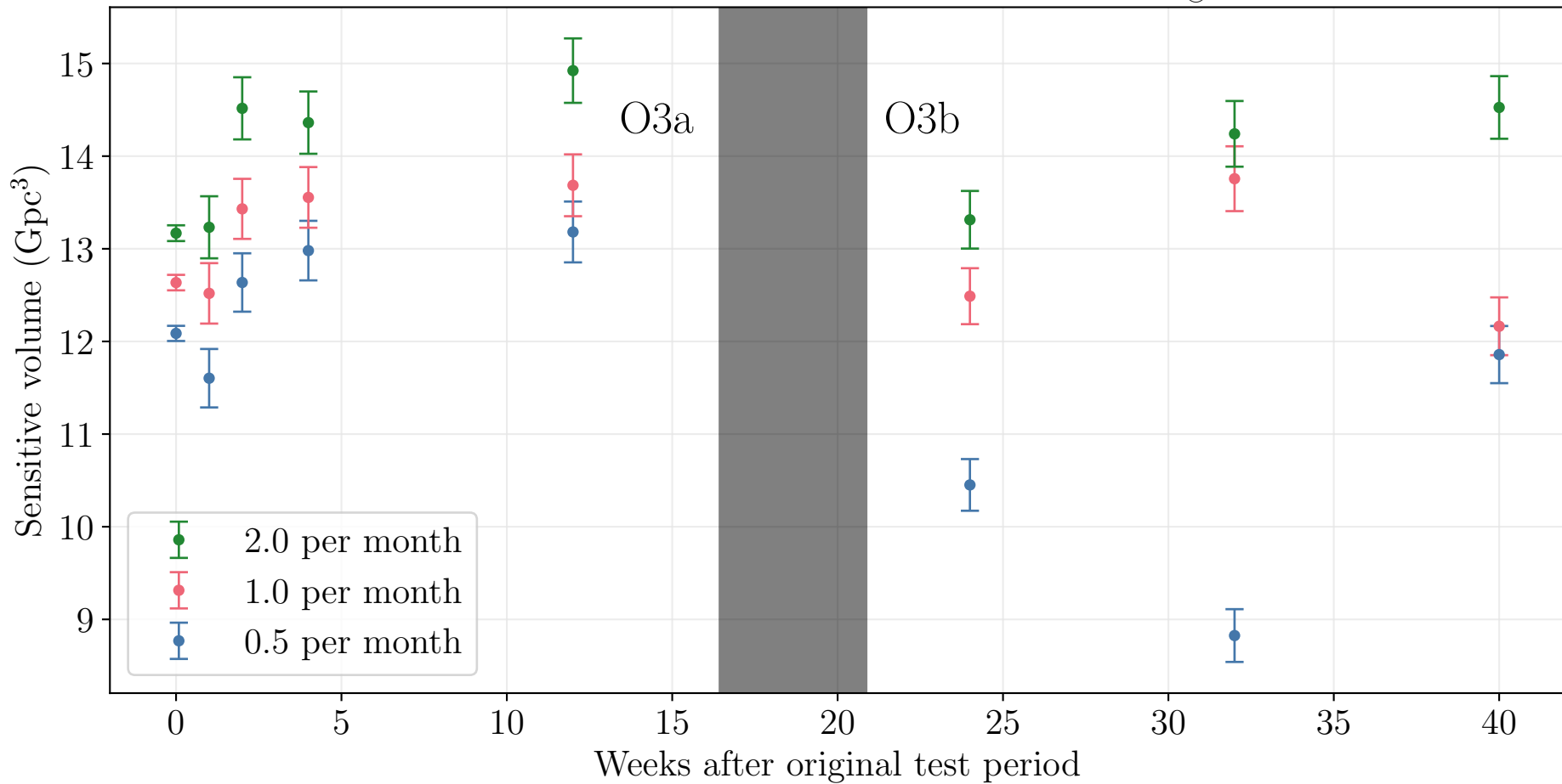
Sensitive Volume Over Time for 35-35 M_{\odot}
