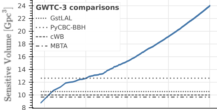
Log Normal m_1 = 20, m_2 = 20
