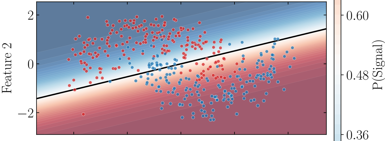
Logistic Regression acc = 84.0
