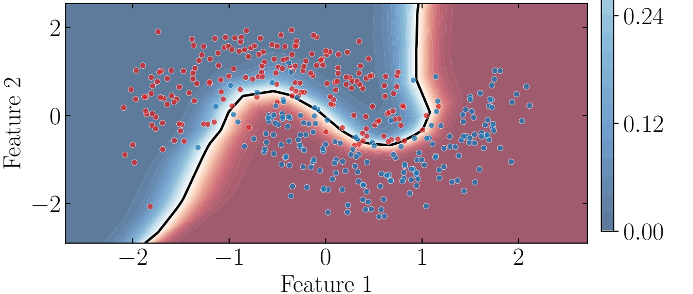
Neural Network acc = 94.0
