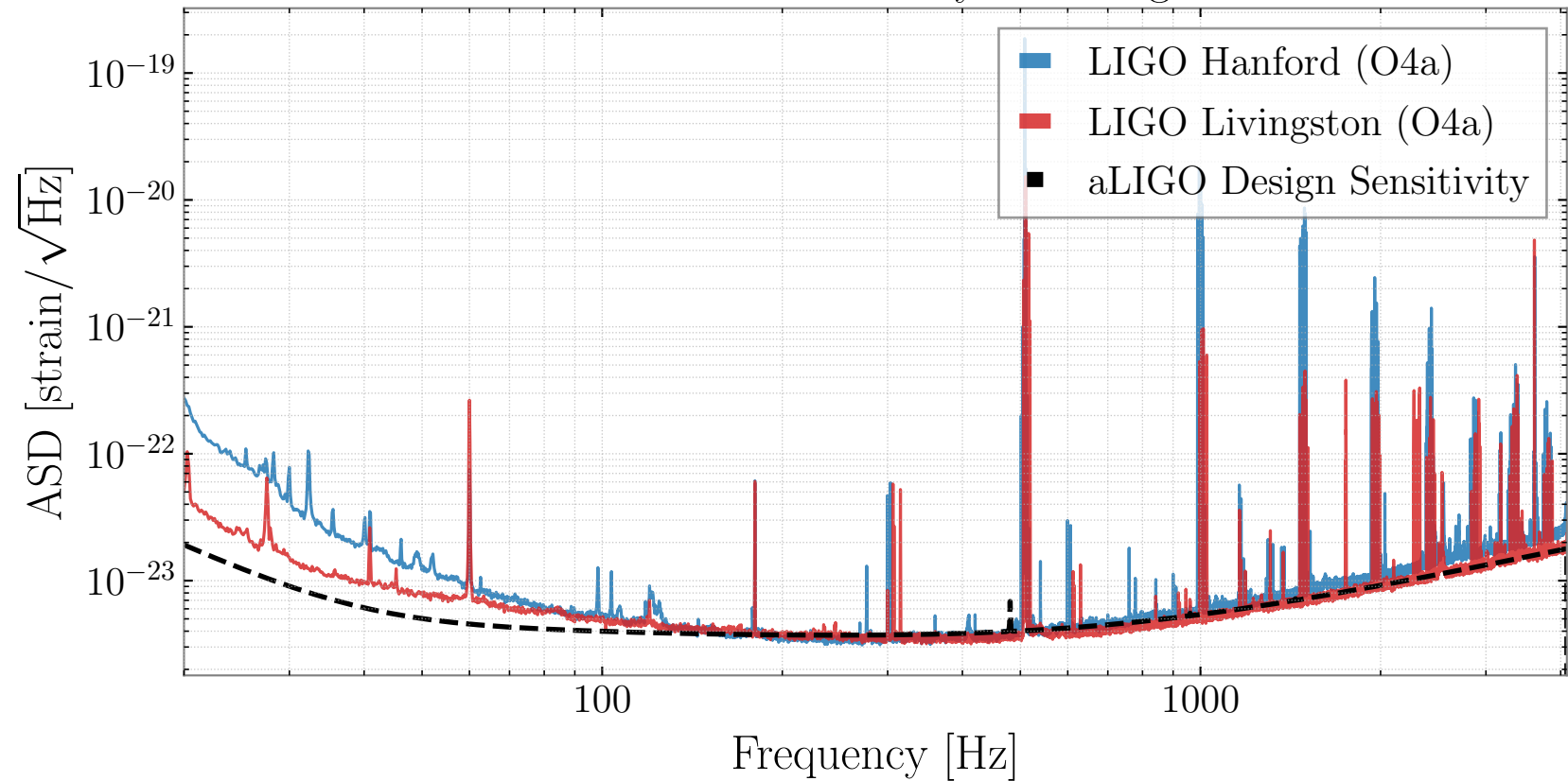
LIGO O4a Sensitivity vs. Design
