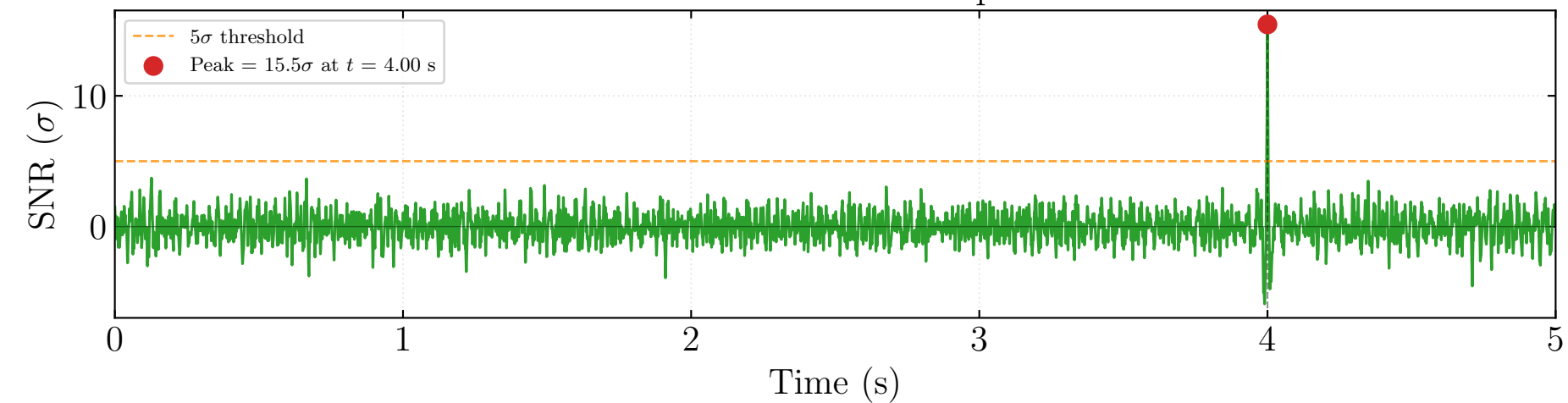
Matched Filter Output
