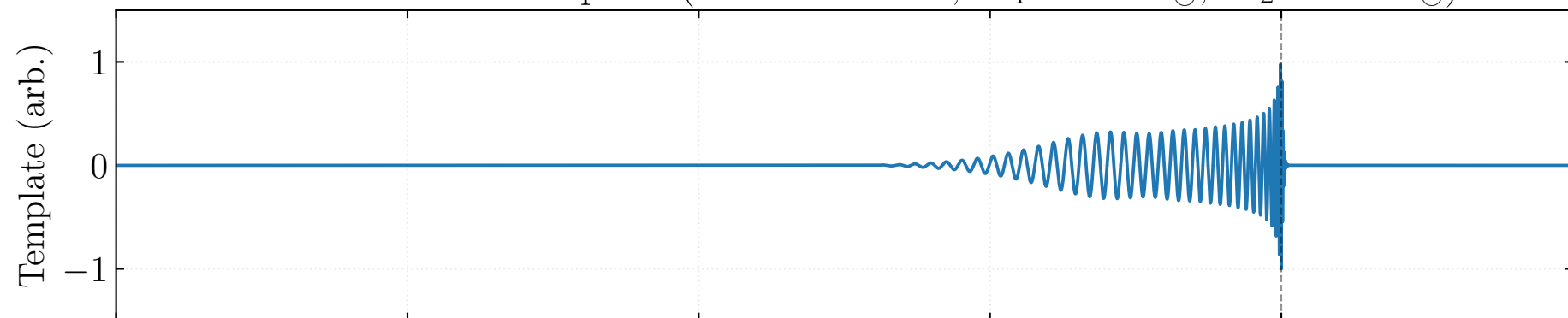
Matched Filter Template (IMRPhenomD, m_1 = 36 M_\odot , m_2 = 29 M_\odot )
