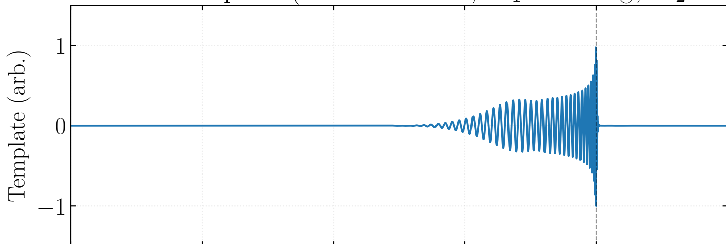
Matched Filter Template (IMRPhenomD, m_1 = 36 M_\odot , m_2 = 29 M_\odot )
