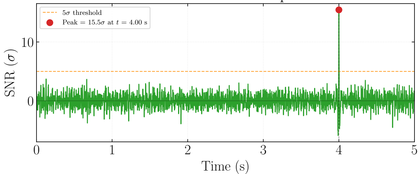
Matched Filter Output
