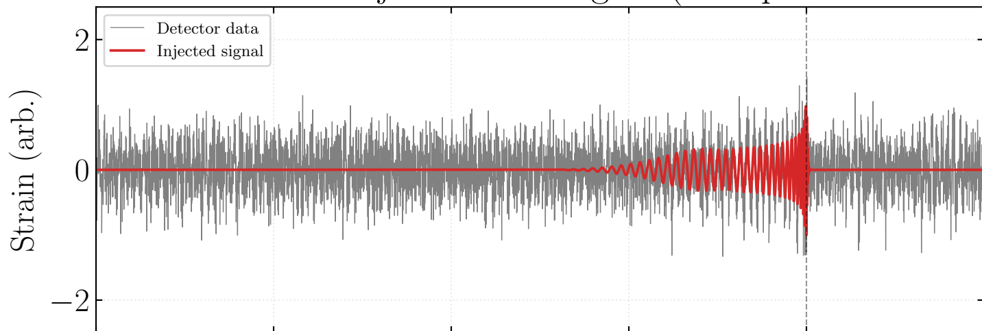
Detector Data with Injected GW Signal (bandpassed 20–500 Hz)
