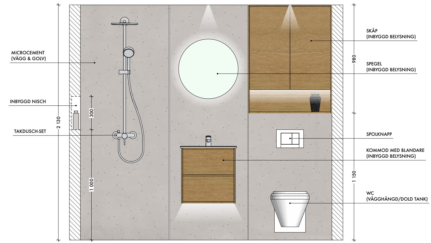
ELEVATION 1 1:20
