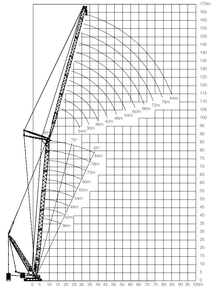
7. Super-lift tower jib lifting characteristic curve
