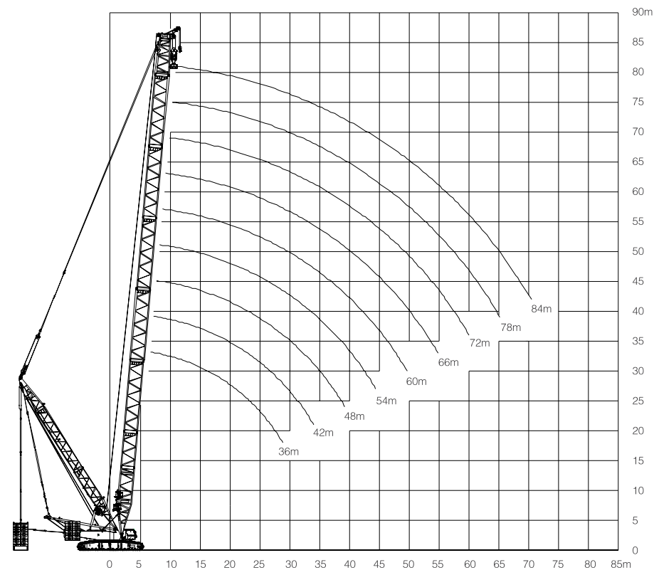
5. Super-lift boom lifting characteristic curve
