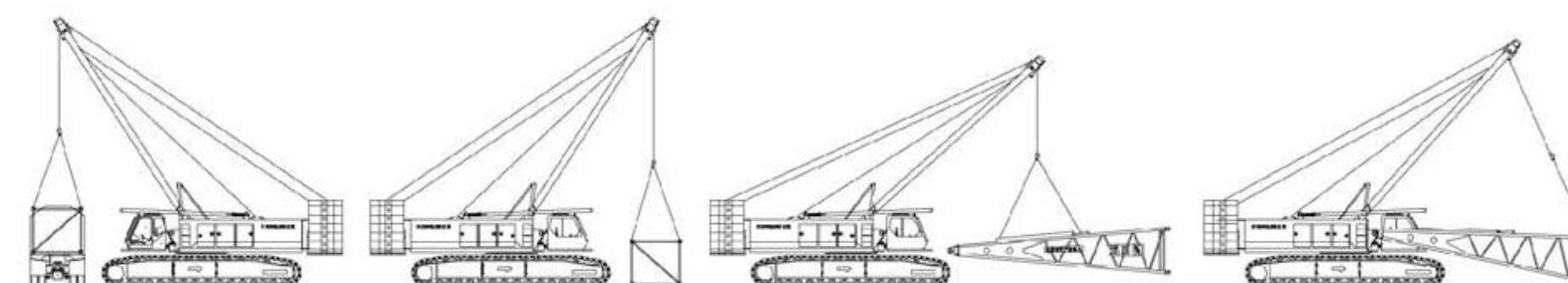
Unloading and assembly of boom
