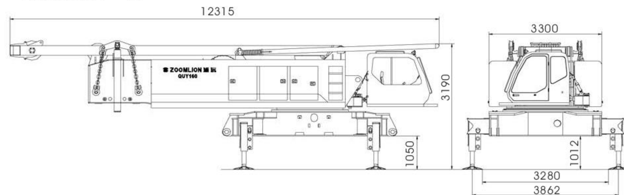
Basic machine---46t
