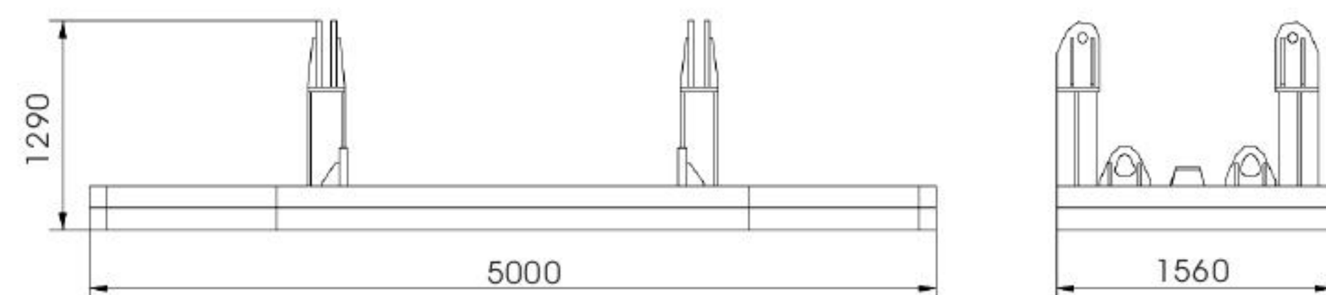
Counterweight---4.45t×12
