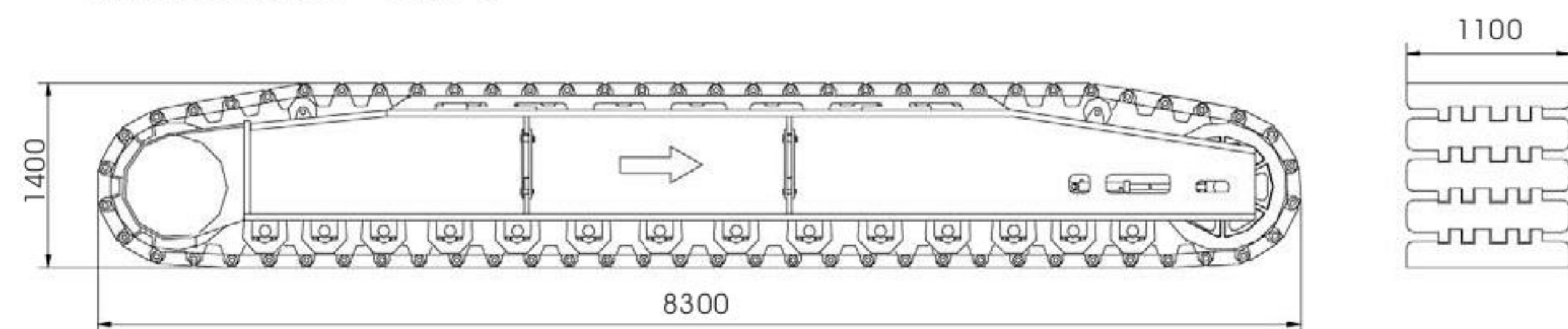
Crawler side frame---18.4t×2
