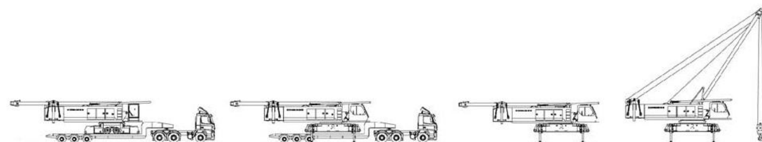
Unloading of basic machine
