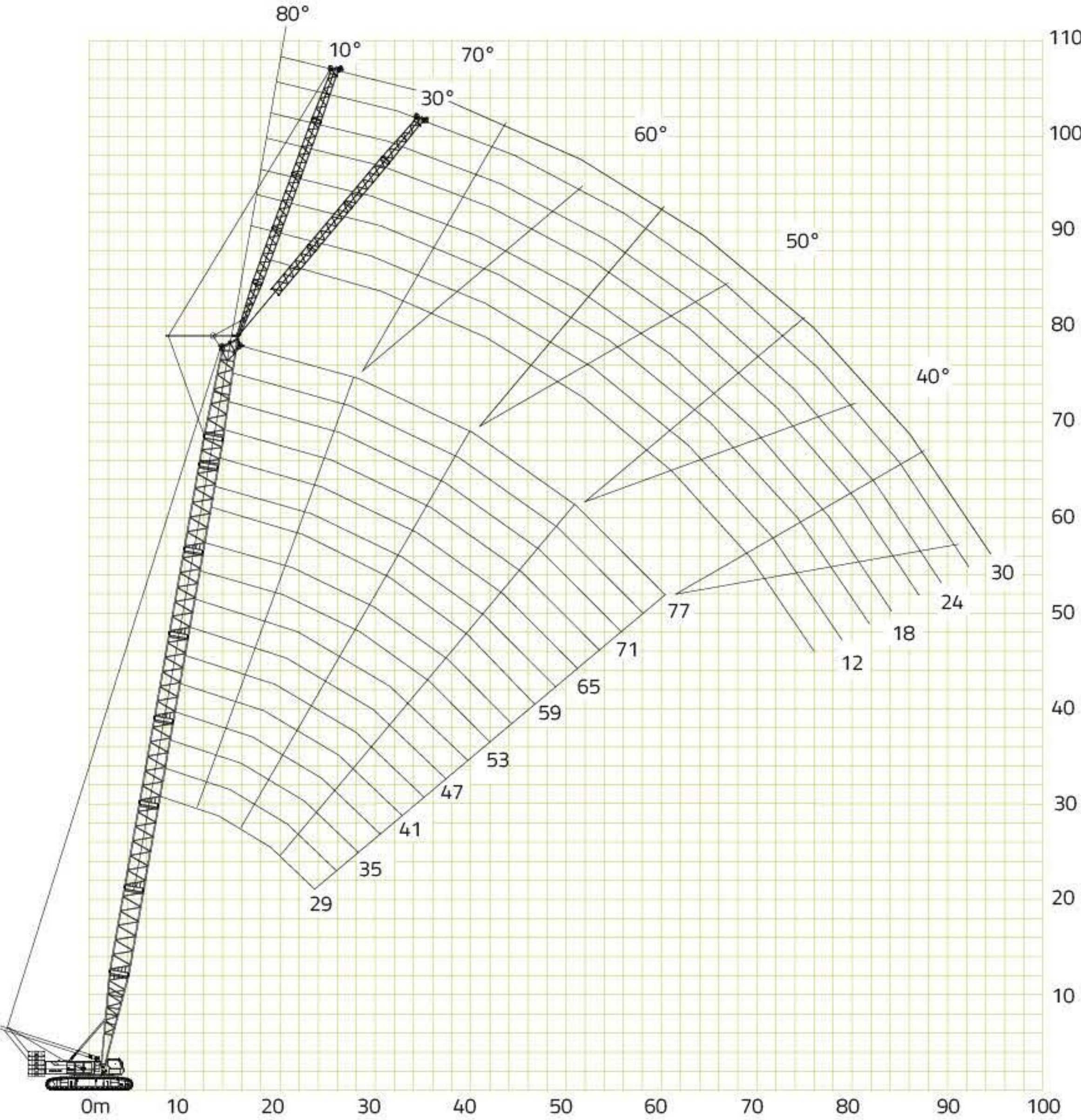
Fixed Jib Lifting Height Curve
