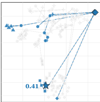
(a) Population Search (LoCoMo)
